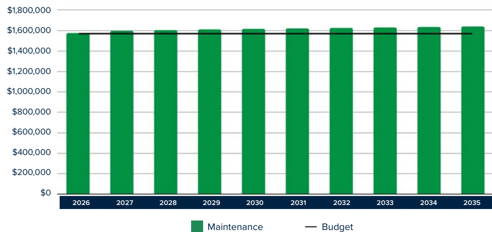
Figure 4.1.4: Operations and Maintenance Summary – Transport
