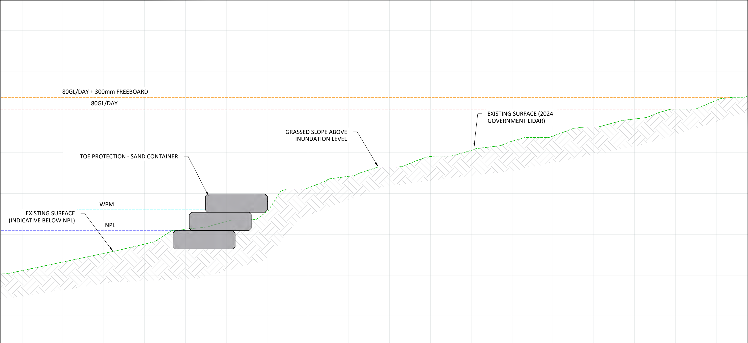
TYPICAL SECTION - OPTION A
