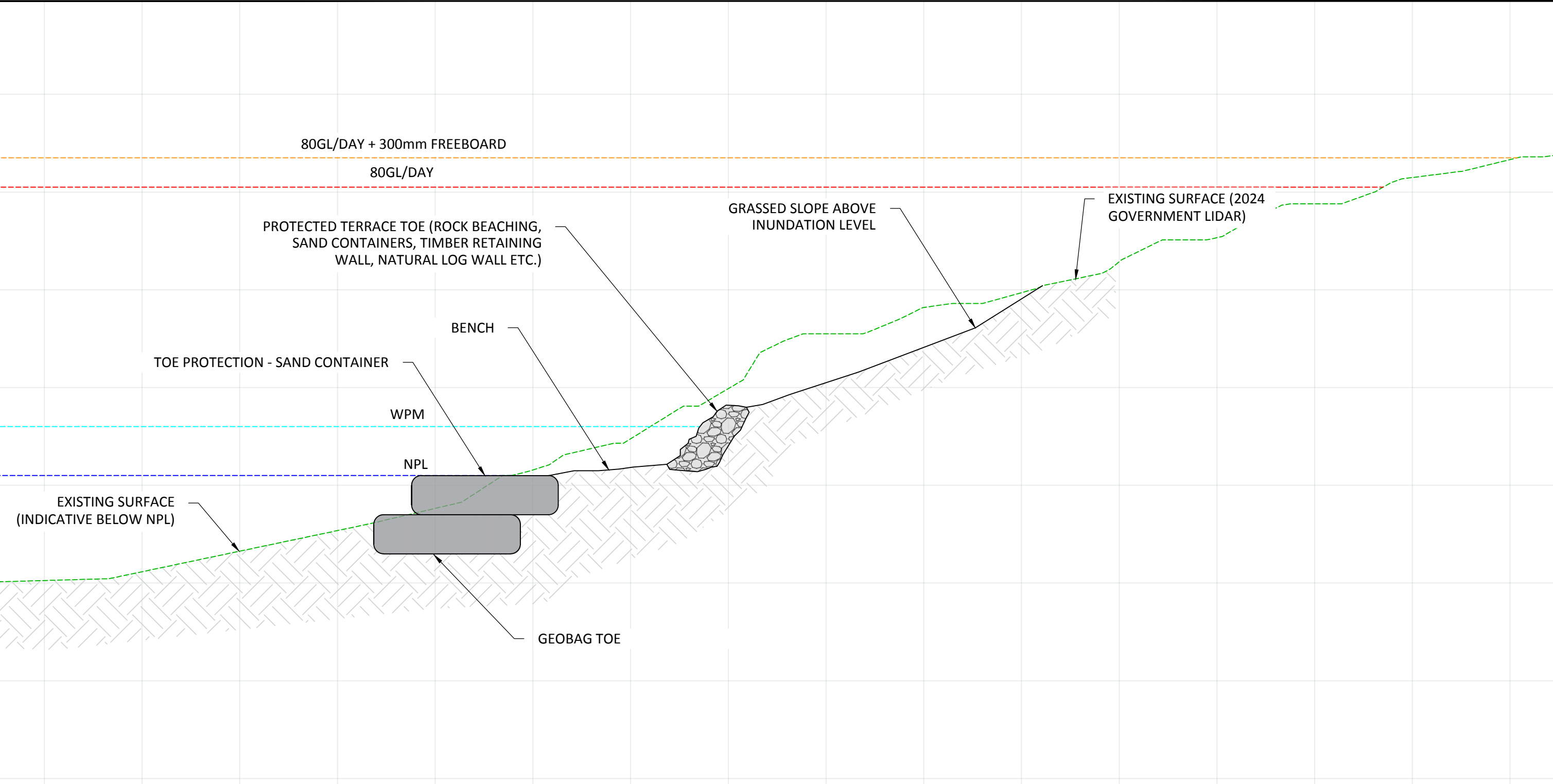
TYPICAL SECTION - OPTION B
